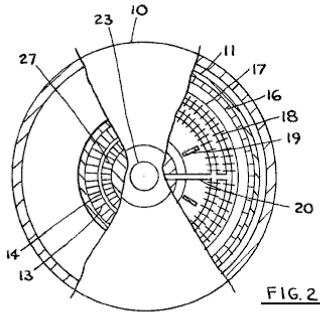
Fig.2 shows an end view of the unit of Fig.1 where 10 is the casing, 11 is the first rotor, 17 is the second rotor, 16 are the first-fluid nozzles, 18 is a heat exchanger, 19 are vanes, 20 is a conduit, 13 , 14 and 27 form a heat exchanger for the first-fluid and 23 is the second rotor shaft.
